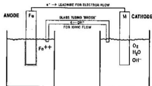
Fig.3 Corrosion Cell in Reinforced Concrete.
