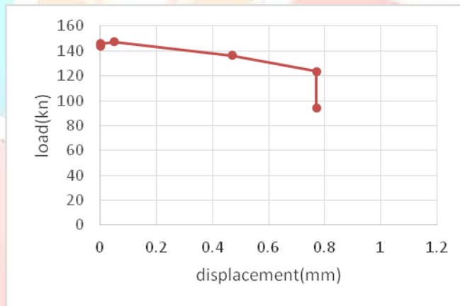
Graph 2 Load vs Deflection for 28 days conventional.
