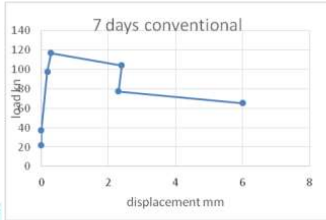
Graph 1 Load vs Deflection for 7 days conventional.
