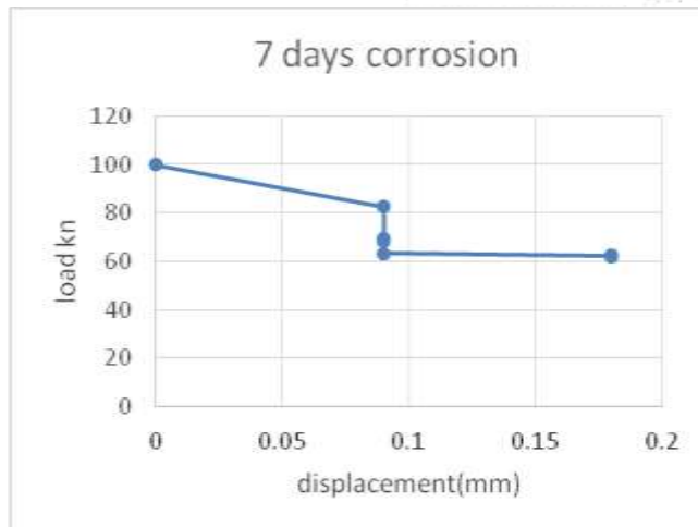
Graph 3 Load vs Deflection for 7 days corrosion.
