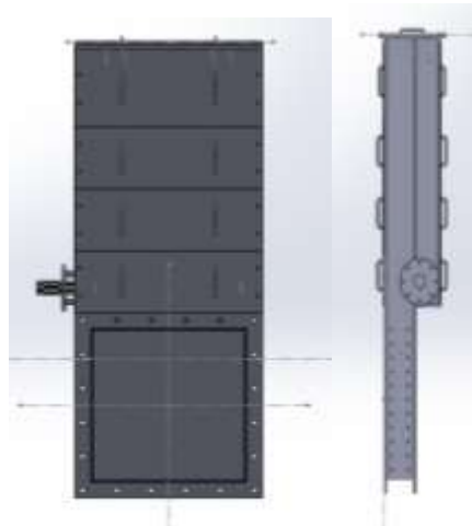
Fig.2. Front view & Side view of Guillotine Damper
