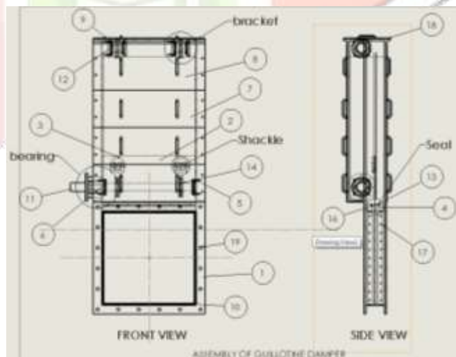
Fig.1 Orthographic view of Guillotine Damper assembly
