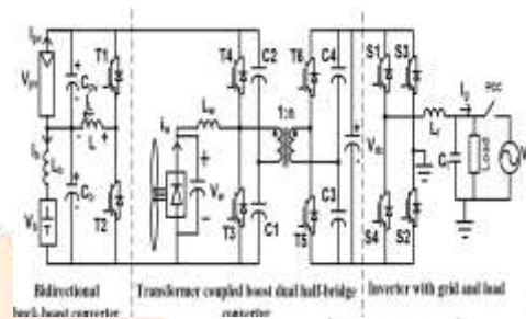
Fig.1 Proposed converter configuration
