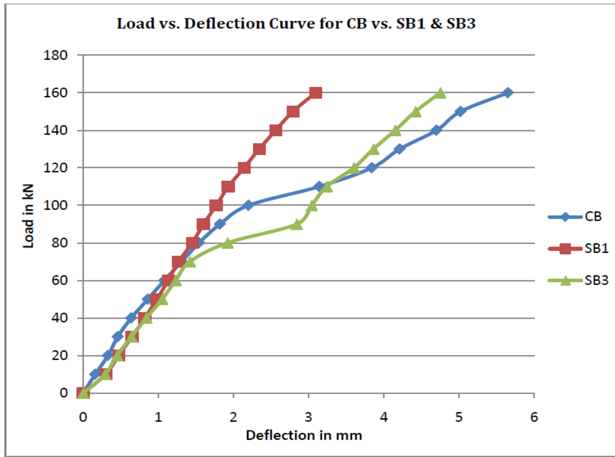
Figure: One of the results obtained by author by comparing control beam and strengthened beam
