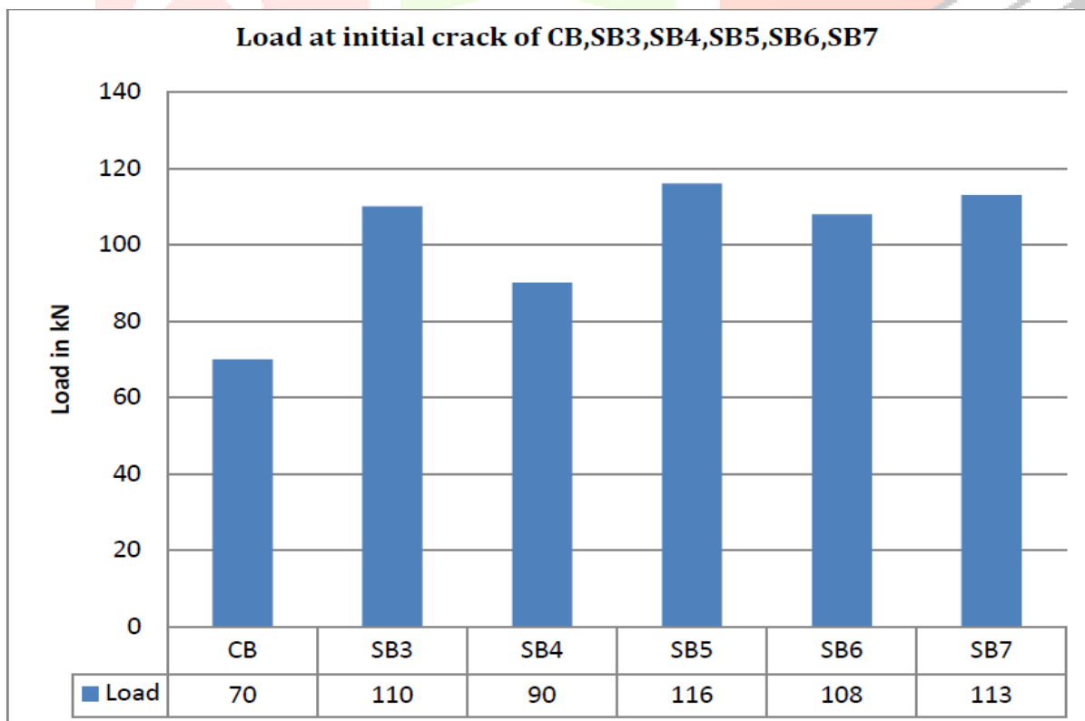
Figure: One of the results obtained by author by comparing control beam and strengthened beam
