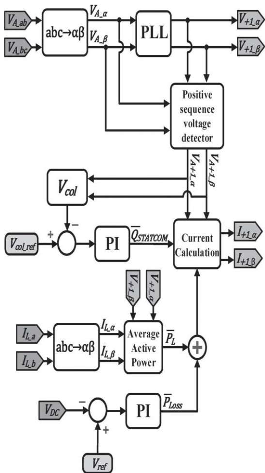
Fig.3. Novel iUPQC controller.
