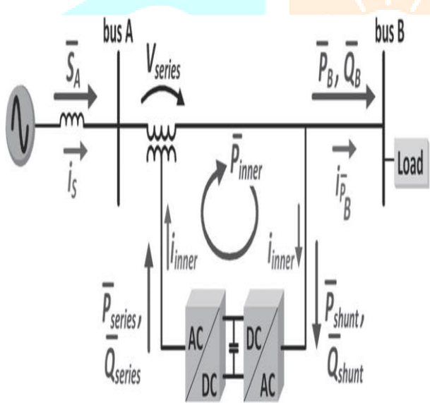
Fig. 4. iUPQC power flow in steady -state.
