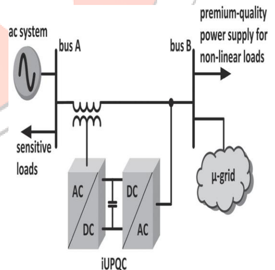
Fig.1. Example of applicability of iUPQC.
