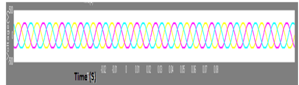
Fig. 8. iUPQC transitory response during the connection of a three phase diode rectifier: (a) load currents, (b) grid currents, (c) load voltages and (d) grid voltages.
