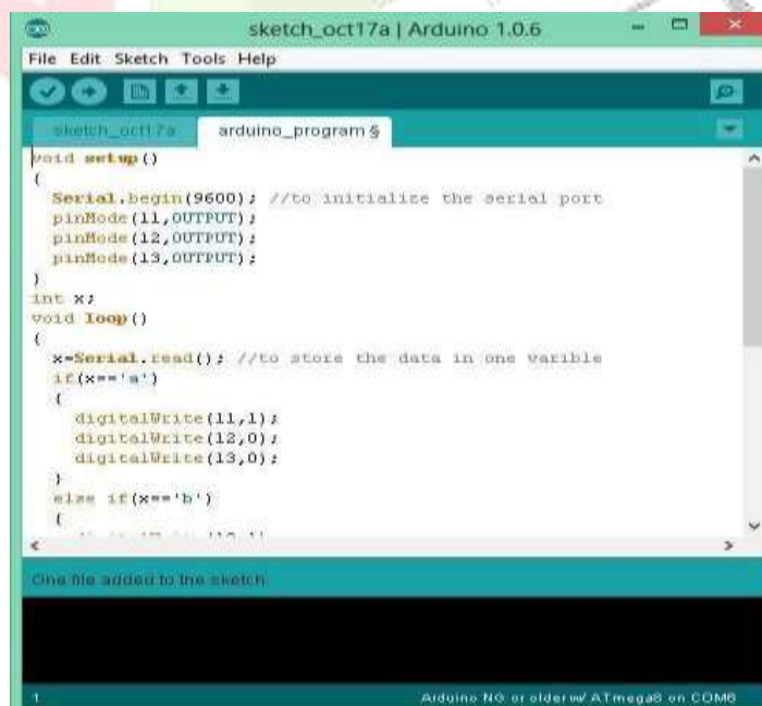
Figure 6: Arduino IDE
