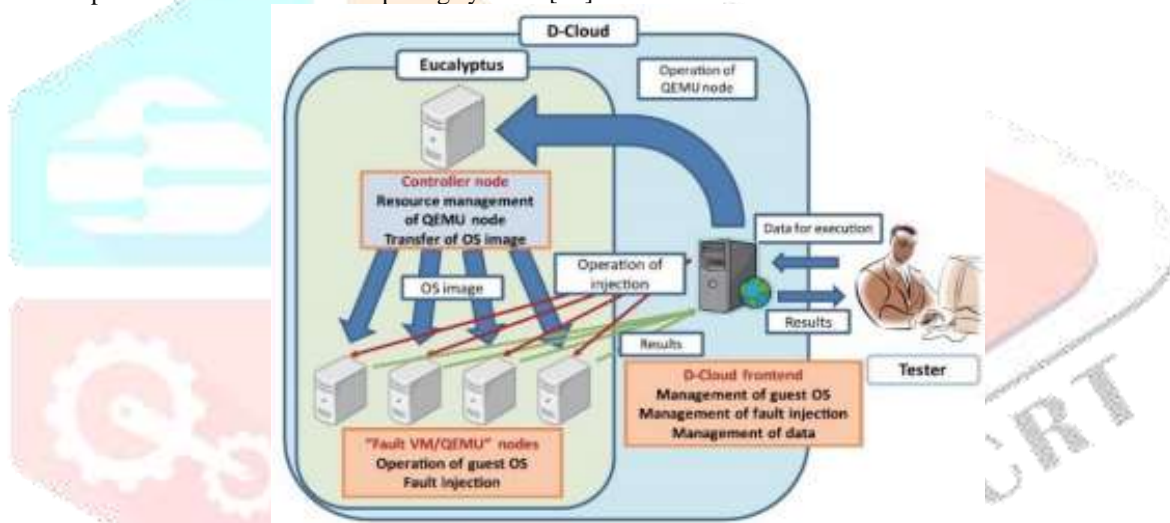
Fig. 5. Architecture of D-Cloud
