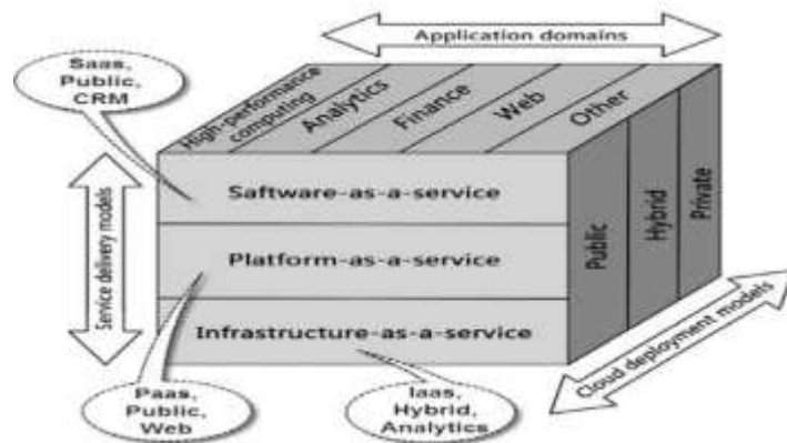
Fig. 1. Cloud computing services and deployment models
