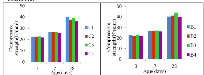
Fig. 6. (a). Compressive strength of normal concrete with RHA and QD
