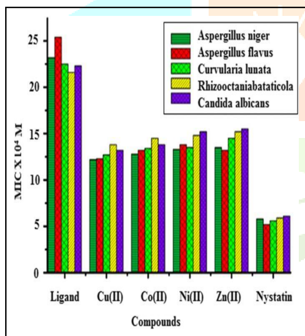
Figure1.12: The antifungal activity of the synthesized compounds
