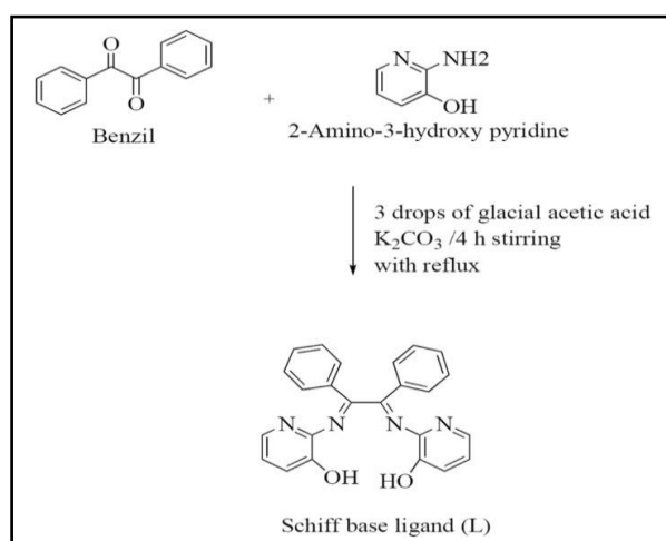
Figure 1: Synthesis of Schiff base ligand
