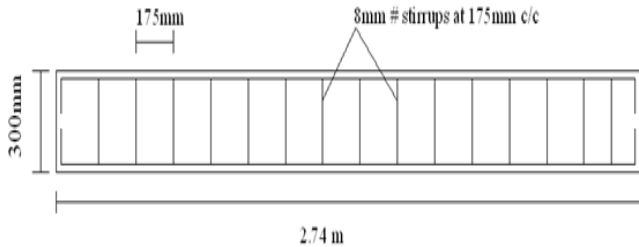
Fig. 1 Reinforcement details of beam elevation
