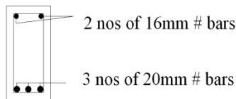
Fig. 2 Reinforcement details of beam section
