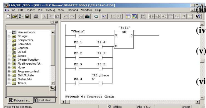
Fig 1: Siemens PLC programming tool in LD.
