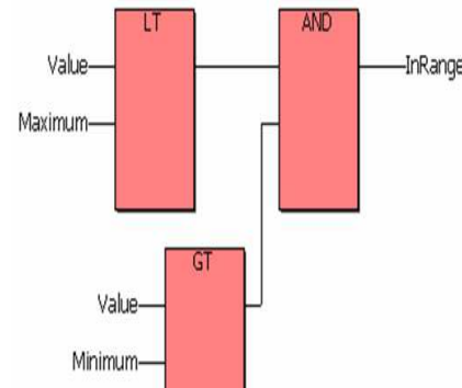
Fig 2: Example of FBD.
