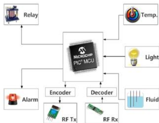
Fig. 3 Block diagram of Slave-1 module.
