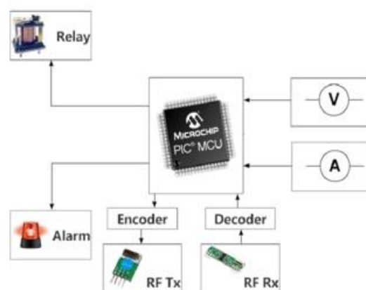
Fig. 4 Block diagram of Slave-2 module.
