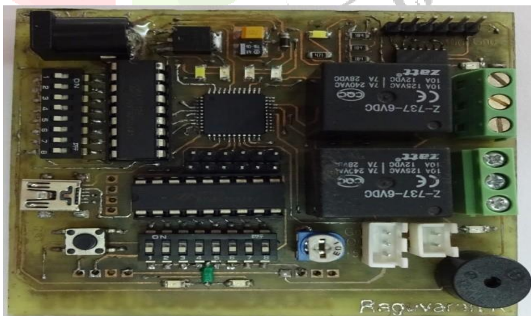
Fig. 6 Top side of slave-1 hardware
