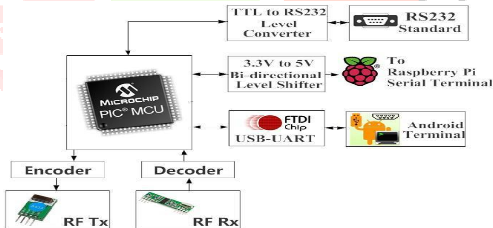
Fig. 2 Block diagram of master module.
