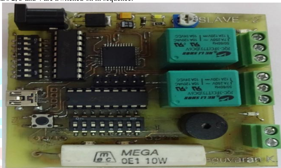
Fig. 7 Top side of slave-2 hardware
