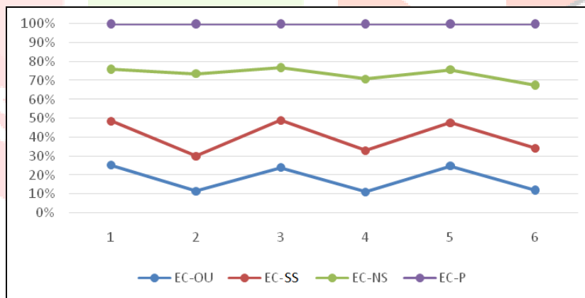
Figure 2. Keeping 341-bit prime value fixed for all schemes
