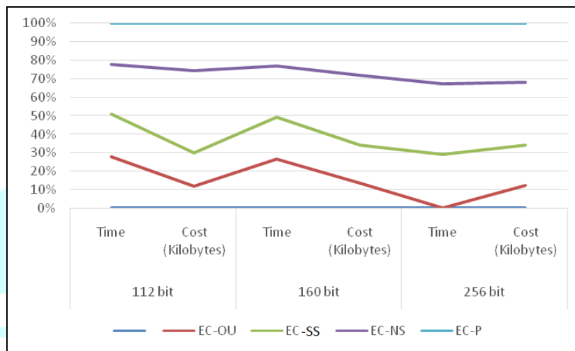
Figure 1. Secure Multiparty addition using various ECC-based Encryption Schemes
